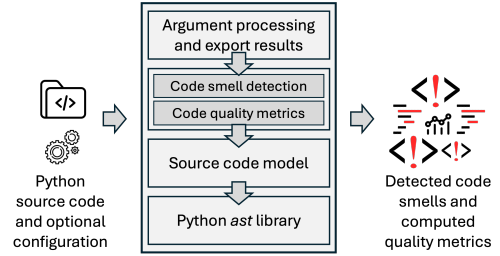
Fig. 1. Architecture of DPY tool.
